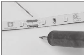
Splice Connection
