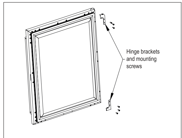
Figure 10. Door Brackets
