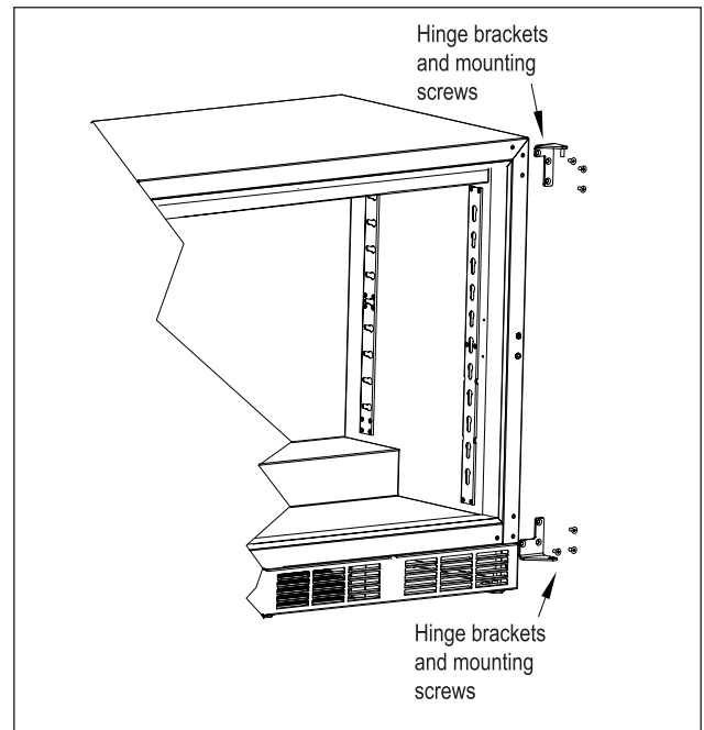
Figure 9. Hinge Installation
