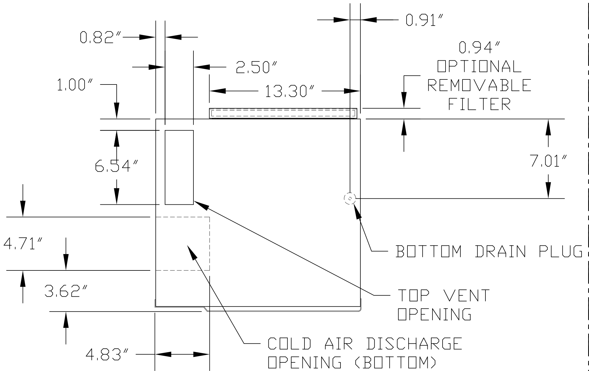
TOP VIEW
